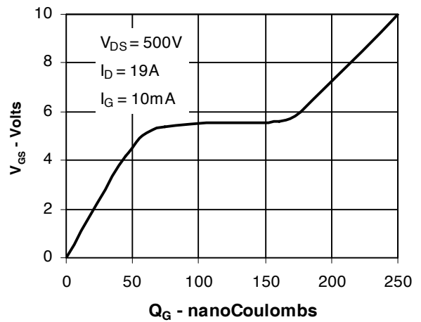
Fig. 10. Gate Charge
